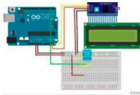
Gambar 1: sensor suhu
